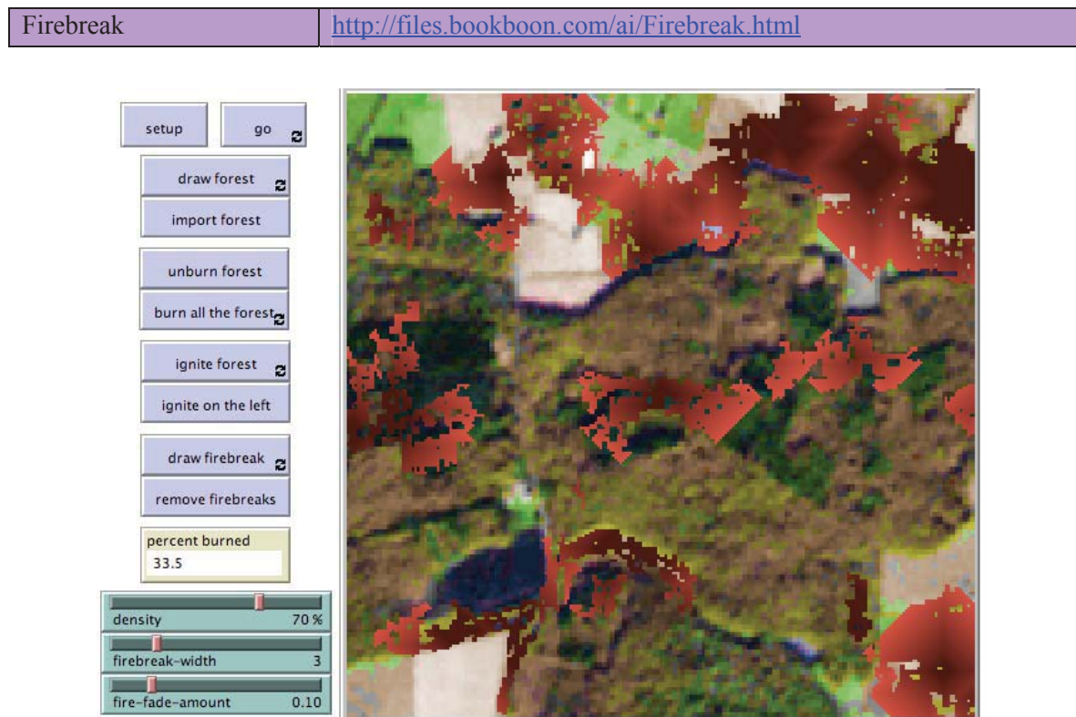
Figure S-6.1.2. Screenshot of the Interface for the Firebreak model after the setup button has been pressed followed by the import-forest and burn all the forest buttons, with the slider values as shown in the image.
