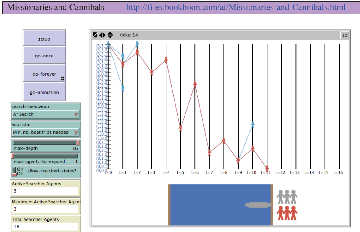
Figure 8.2.2. Screenshot of the Interface for the Missionaries and Cannibals model for after the setup button has been pressed followed by the go-forever button and then the go-animation button, with the slider values as shown in the image.
