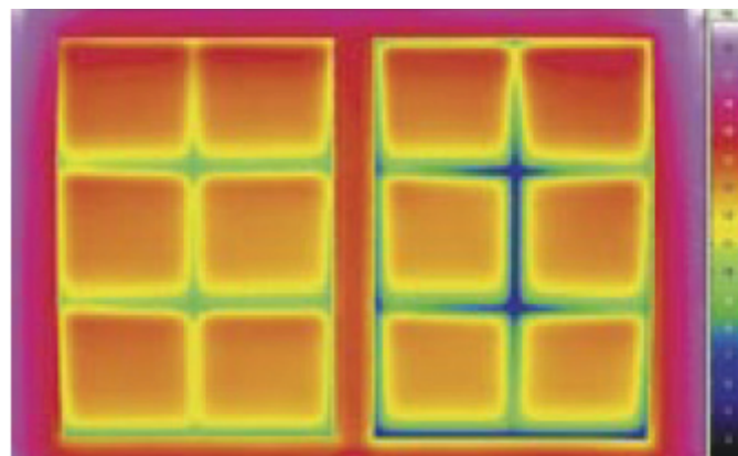
Figure 34. Infrared photo of two windows with Swisspacer to the left and normal Al profile to the right. From www.scanglas.dk/servlet/RichTextHandler?name=swisspacer.pdf .
