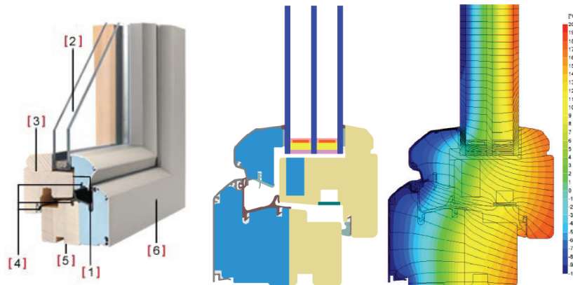
Figure 22. Example of a wood window frame with insulation filled Al cladding with low U-value - ed[if]ition passiv by Internorm International GmbH. One photo/drawing to the left, one schematic drawing in the middle and one temperature profile to the right. Wood frame with PUR and PUR filled Al cladding. Frame U-value U_f = 0.73 \text{ W/m}^2\text{K} . Compare with fixed window in Figure 27. From http://www.passiv.de and www.internorm.com .
