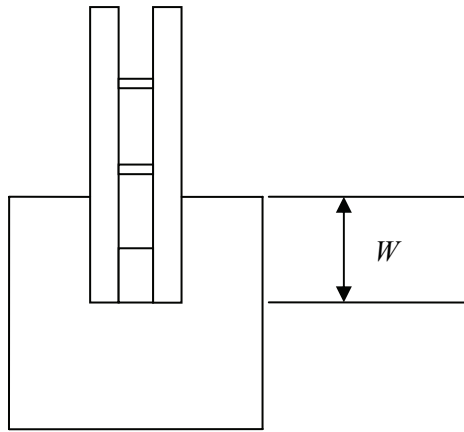
Figure 9. Schematic showing of a vacuum glazing with a wood frame. W is the rebate depth. The size of the pillars separating the glass panes in the figure is not comparable to a real vacuum window.
