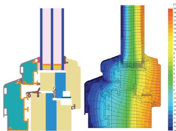
Figure 21. Example of a wood window frame with insulation filled Al cladding with low U-value - KombiRoyal Plus PH by NIVEAU Fenster Westerbürg GmbH. One schematic drawing to the left and one temperature profile to the right. Wood frame with PUR and XPS filled Al cladding. Frame U-value U_f = 0.68 \text{ W/m}^2\text{K} . From http://www.passiv.de and www.niveau.de .
