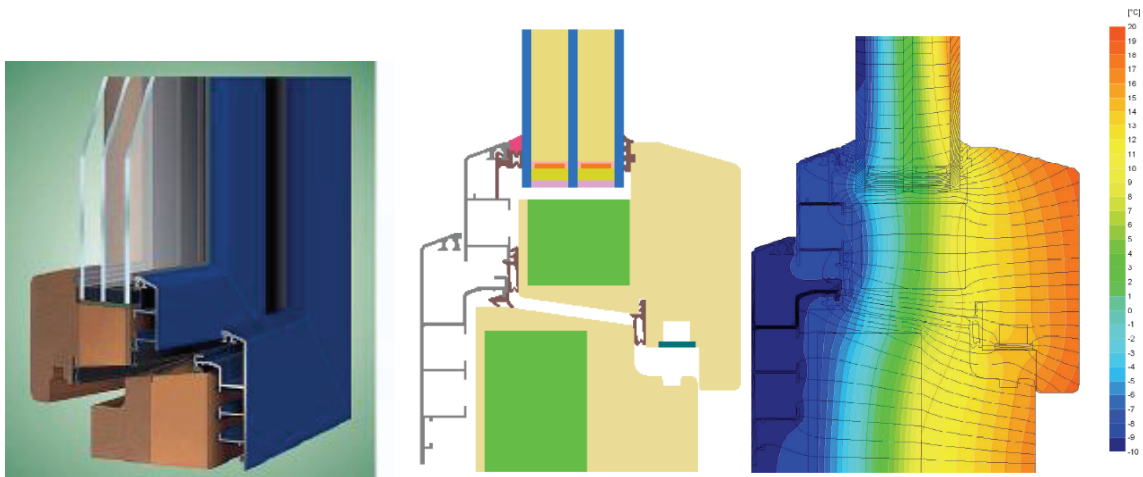
Figure 17. Example of a wood window frame with low U-value - Super-Warmfenster U 07 Serie HF 8120 by HEUSER Türen + Fenster-Metalbau GmbH. One photo to the left, one schematic drawing in the middle and one temperature profile to the right. Wood frame with PUR. Frame U-value U_f = 0.65 \text{ W/m}^2\text{K} . From http://www.passiv.de and www.heuser-tueren-fenster.de .
