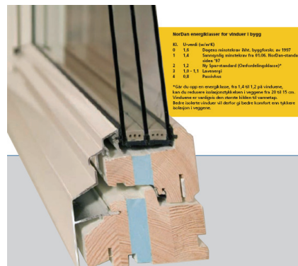
Figure 19. Example of a wood window frame with low U value - N Tech Passiv Superspacer by NorDan AS. Wood frame with PUR. The frame U-value is not stated, whereas the total window U-value is reported to be U_w = 0.7 \text{ W/m}^2\text{K} . From http://www.nordan.no .
