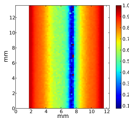
Figure 5.3: The visibility from scan 109 of the diffraction pattern is highest at the edges of the sample, and slowly decreasing towards the center. This is consistent with Figure 5.2, where there was no preferred orientation at the center, which was located to the right of the symmetric center of the dog-bone. One can see some dark red pixels at the center, which is most likely caused by a failure in the analyzing routine, because of the lack of preferred scattering direction.
