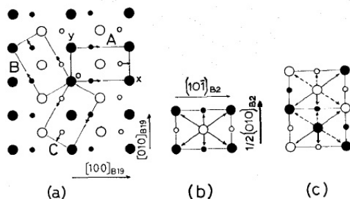
FIG. 9: The reverse transformation from a HCP into a BCC structure is accomplished by a contraction along the x -direction and an expansion along the y -direction so that the ratio \Delta x/\Delta y becomes \sqrt{2} in cell A . This is followed by a shuffling indicated by the small arrows. In (a) the three possible lattice correspondences are shown, A , B and C . The atomic configurations obtained by the reversed transformation for the variants A in (b) and B in (c). The projection plane is the (101)_{bcc} plane. The larger and smaller circles represent atom positions in alternate (101)_{bcc} planes. The arrows indicated by solid and broken lines represent unlike and like atoms in the nearest neighbor positions, respectively 5 .
