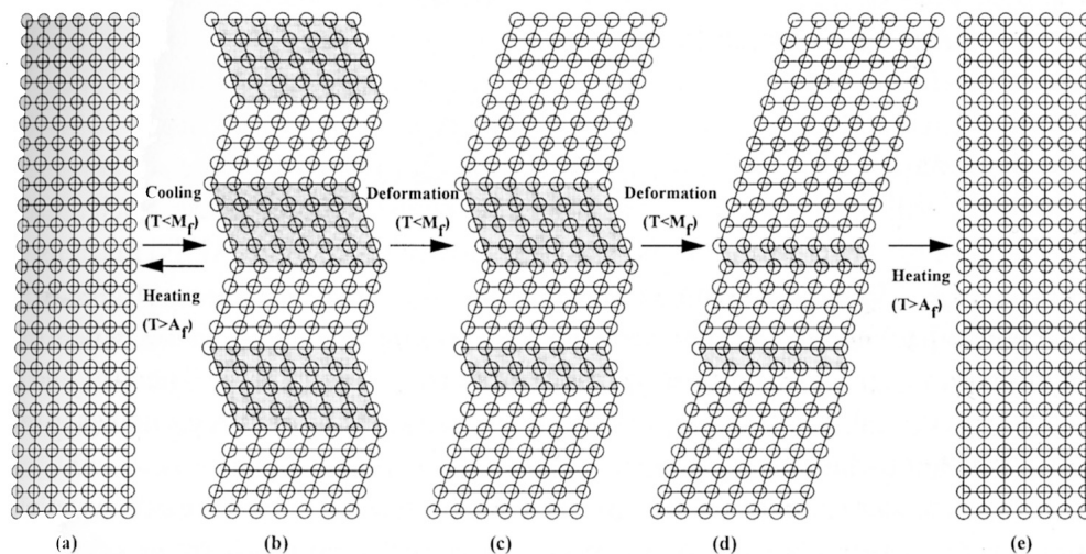
FIG. 10: The shape memory effect illustrated. Starting with the original parent single crystal (a), that is transformed into a self-accommodated martensite (b). The deformation in the martensite proceeds by the growth of one variant at the expense of the other (c-d), i.e. twinning or detwinning. Upon heating above A_f , each variant reverts to the parent phase in the original orientation by the reverse transformation.
