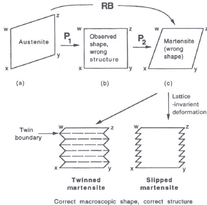
FIG. 6: Illustration of the phenomenological theory of martensite crystallography.
