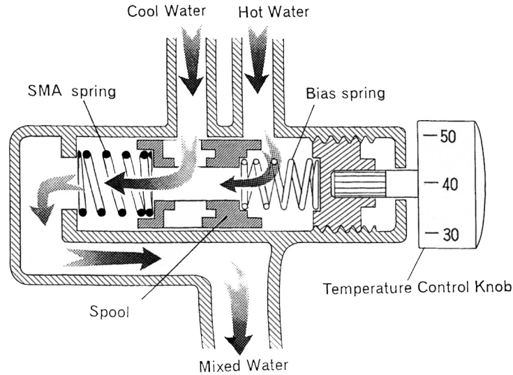
FIG. 18: Sketch of a thermal mixing valve with a shape memory spring. 12
