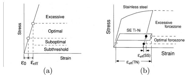
FIG. 17: Schematic stress-strain curves: (a) for an elastic dental arch wire with a high elastic modulus, where the effective strain range corresponding to the optimal force zone is small. (b) for stainless steel and Ni-Ti wires, where the optimal force zone for the Ni-TI wire is much larger than for the stainless steel wire. 12
