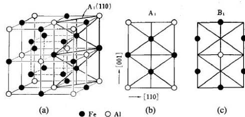
FIG. 2: The crystal structure of the B2 type structure or \beta_2 parent phase. In (a) we see the unit cell, in (b) the (110) plane is depicted, while (c) shows the (110) plane above and below the plane in (b).
