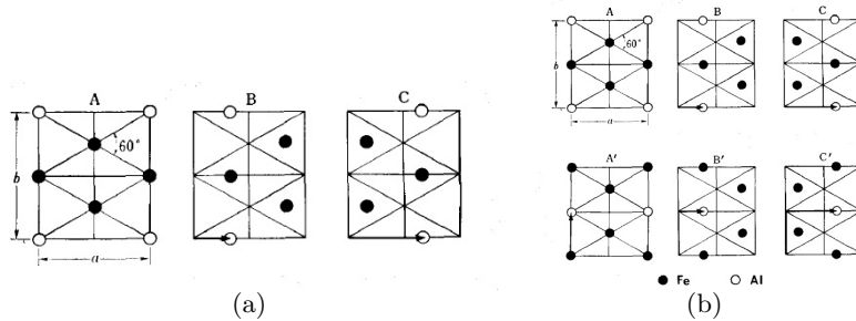
FIG. 7: (a) The three different close packed stacking planes in martensite transformed from a \beta_2 parent phase. (b) By a transformation from a \beta_1 parent phase we get six different close packed stacking planes.
