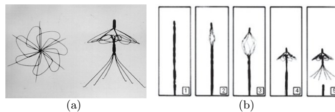
FIG. 14: (a)The Simon filter as it looks when it is expanded in the vein.(from duerig) (b)The procedure of releasing the Simon vena cava filter. Picture 1 shows the filter in it's deformed state inside the catheter. The following pictures shows how the filter expands as it is released from the catheter. In the last picture the filter has returned to its original shape. 6
