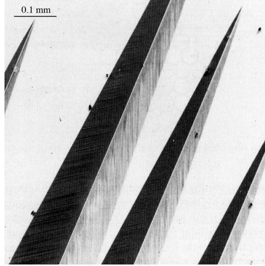
FIG. 1: Optical micrograph of a CuAlNi -alloy. The smooth, light surface of the austenite is contrasted by the platelike martensite.
