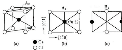
FIG. 2: The crystal structure of the B2 type structure or \beta_2 parent phase. In (a) we see the unit cell, in (b) the (110) plane is depicted, while (c) shows the (110) plane above and below the plane in (b).
