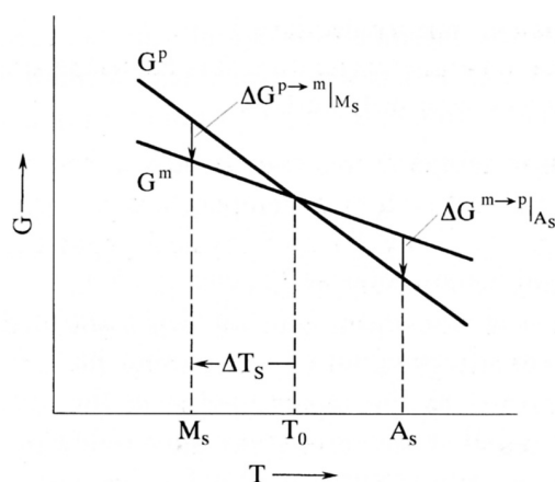
FIG. 8: Gibbs free energy plotted against temperature for the parent phase G^p and the martensite phase G^m . The difference in the chemical free energy, \Delta G , drives the martensitic transformation below T_0 while it drives the reverse transformation above T_0 . From book.
