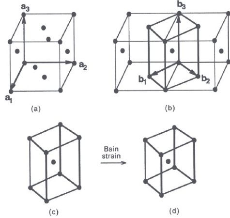
FIG. 4: The austenite lattice shown in (a) is deformed by the Bain strain and is transformed into the BCC martensite lattice shown in (d).
