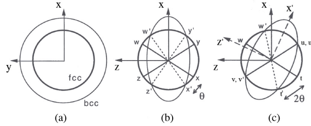
FIG. 5: Illustration of the effect of the Bain strain. When the austenite is undeformed, it is represented as a sphere of diameter wx = yz in three dimensions (a). The strain transforms the parent phase into an ellipsoid of revolution (b). An invariant-line strain is obtained by combining the Bain strain with a rigid body rotation through an angle \theta (c).
