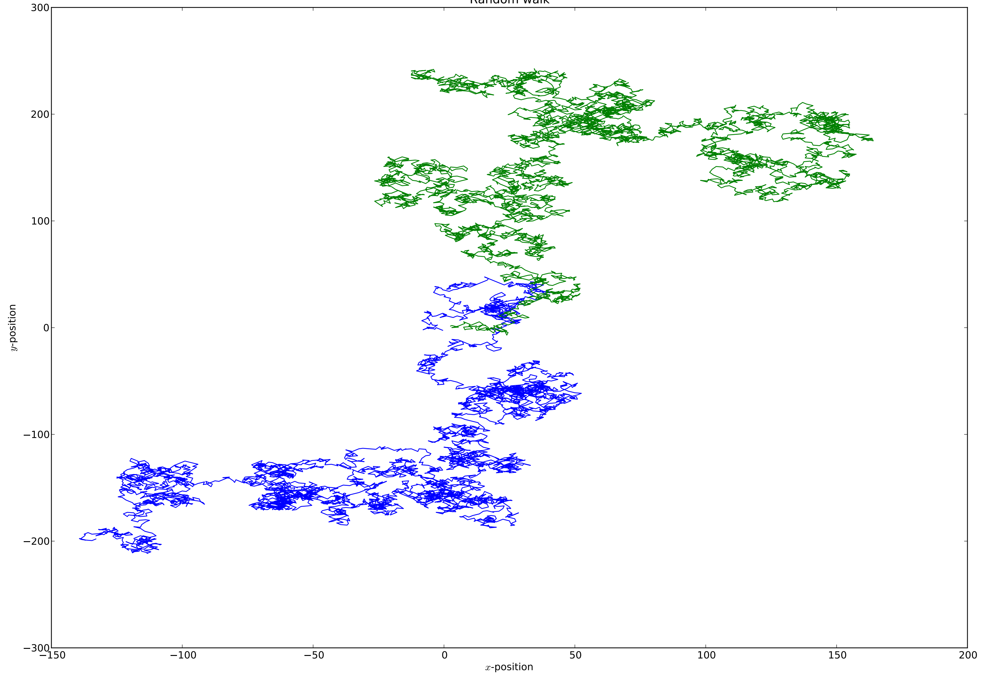
Random walk
