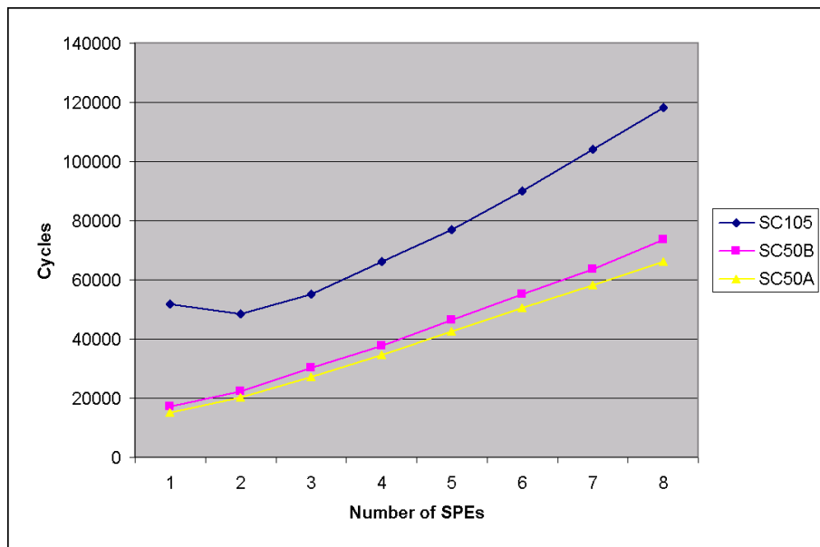
Figure 4.2: Time consumption (in PPE cycles) of parallel SPE standard simplex solver, depending on the number of SPE threads used. Lower is better.
